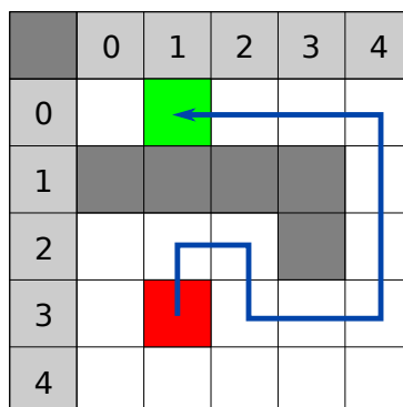
Figure 337: The path taken by the greedy “Best First” algorithm
